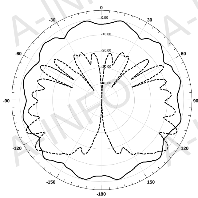
Frequency: 500MHz
