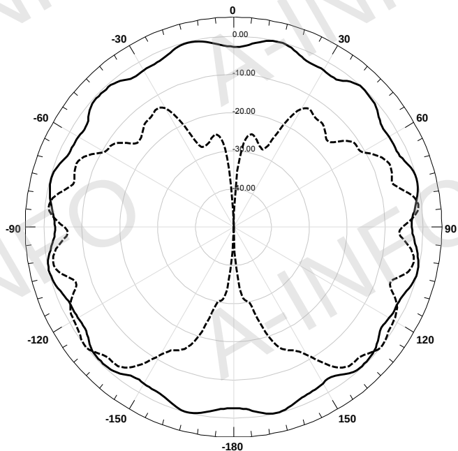
Frequency: 400MHz
