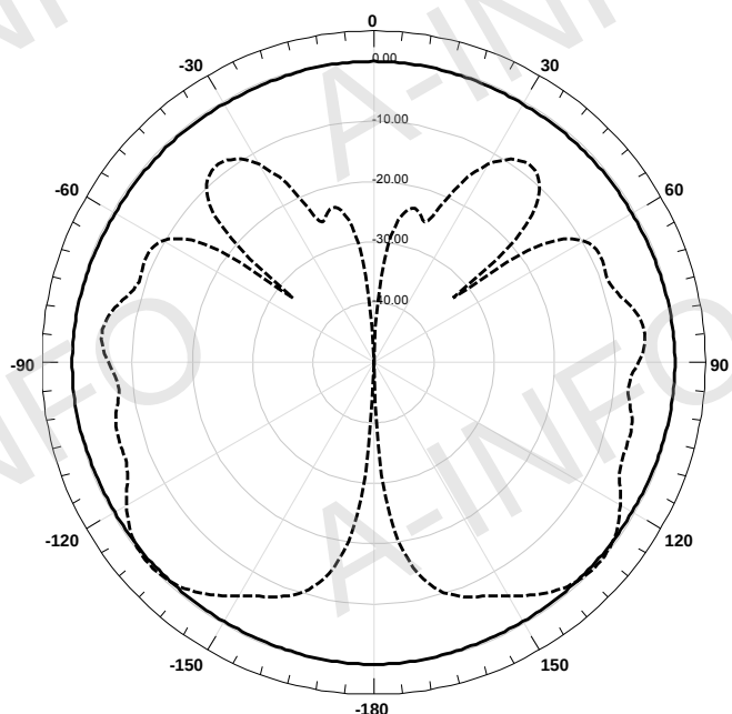
Frequency: 200MHz
