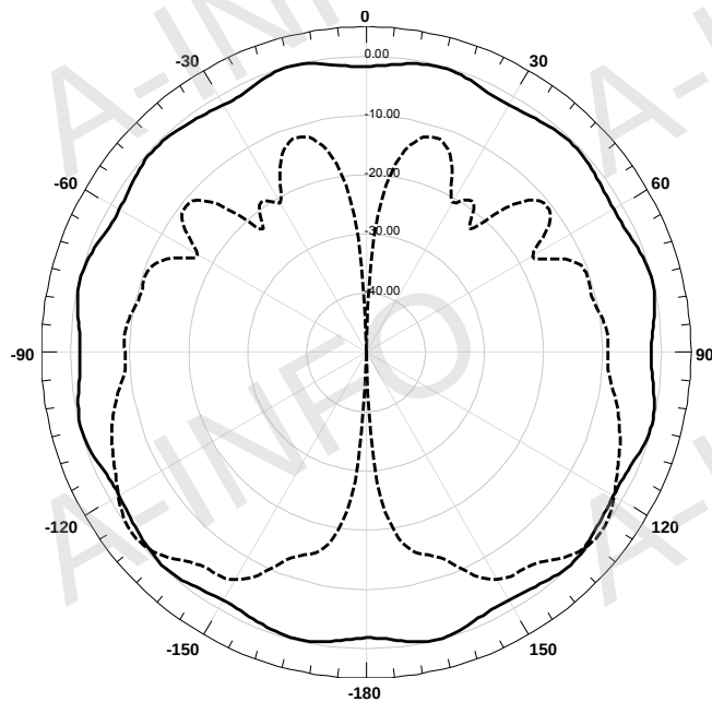
Frequency: 300MHz
